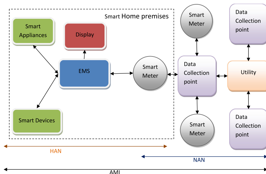
Fig. 5. Interaction of HEMS with various smart entities.
