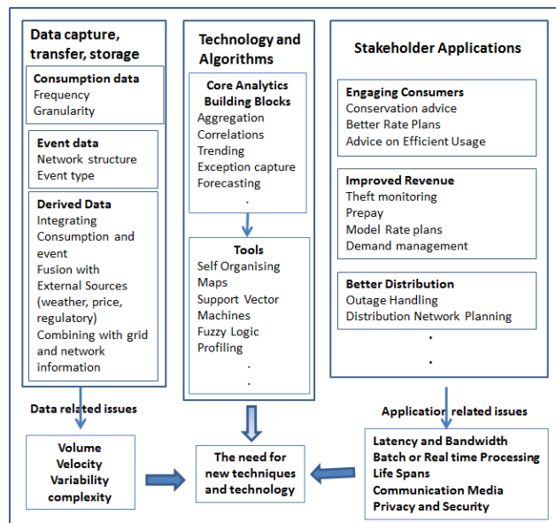
Figure 5: Smart metering framework and new impacts
