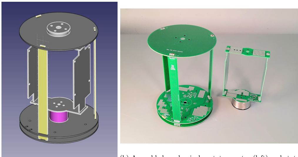
(a) The 3D CAD design of the prototype. (b) Assembled mechanical prototype rotor (left) and stator (right) PCB components.
