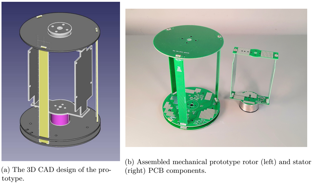
Figure 4: Our prototype IHSM's PCB security mesh design
